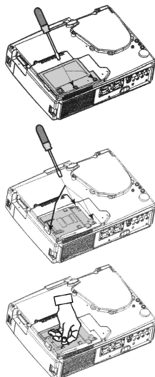
Figure 7: Lamp Replacement
