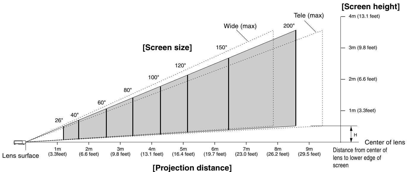
Projection distance and screen height for U3-1100WZ
