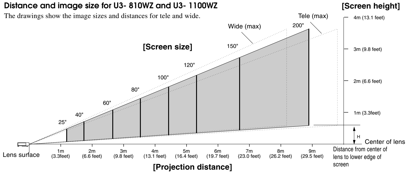
Projection distance and screen height for U3-810WZ
