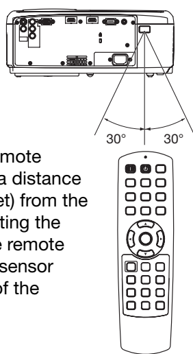
Rear of projector
