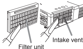
Filter unit
