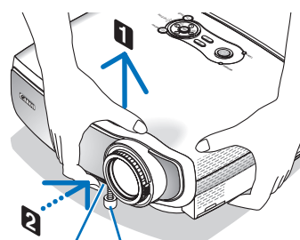
Adjustable Tilt Foot Lock Button
