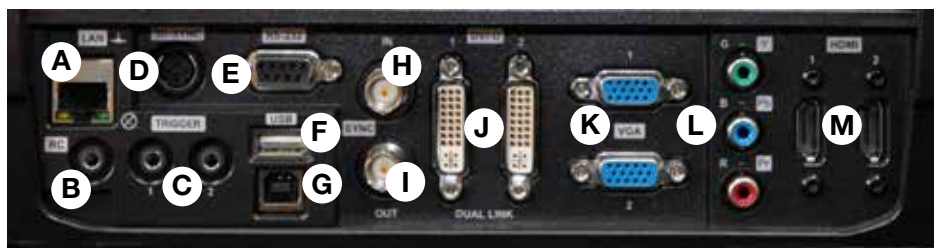
Figure 4-7. Connector panel
