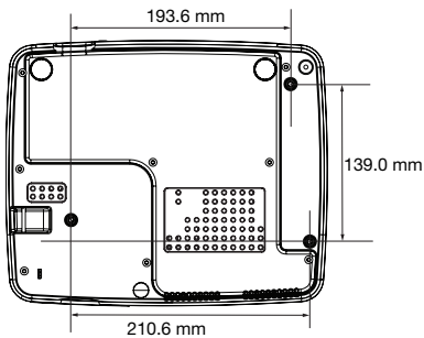
SCREW SPEC. M4 x 8 mm
