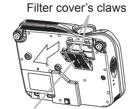
Filter cover
