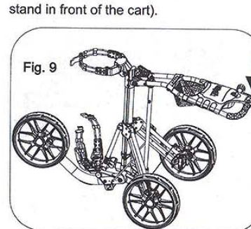
Press the button and rotate the front wheel 180 degree counterclockwise so the front wheel is on the right of the front wheel fork (when you stand in front of the cart).
