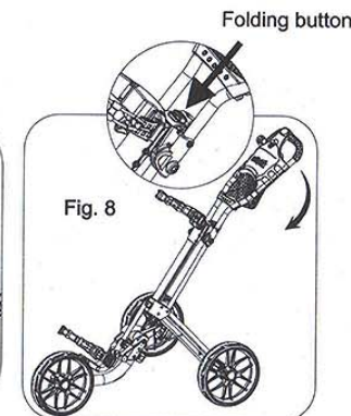
Make sure the handle height adjusting knob is fully tighten .Slightly lift up the handle as Fig. 7 then press the folding button and push the handle downward as shown in Fig. 8 , Fig. 9 to fold the cart till the main frame clicks into the holding slot as in Fig. O.
