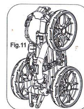
The cart is fully folded.
