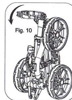
Fold down the upper bag holder bracket
