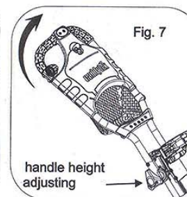
Make sure the handle height adjusting knob is fully tighten .Slightly lift up the handle as Fig. 7 then press the folding button and push the handle downward as shown in Fig. 8 , Fig. 9 to fold the cart till the main frame clicks into the holding slot as in Fig. O.
