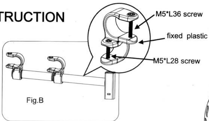
Seat fixed bar and plastic
